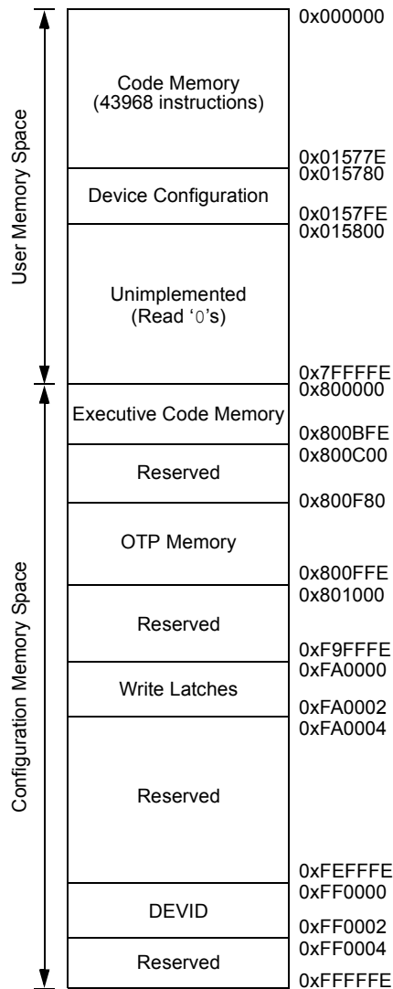
FIGURE 2-8: PROGRAM MEMORY MAP FOR dsPIC33EV128GM00X/10X DEVICES (1)
