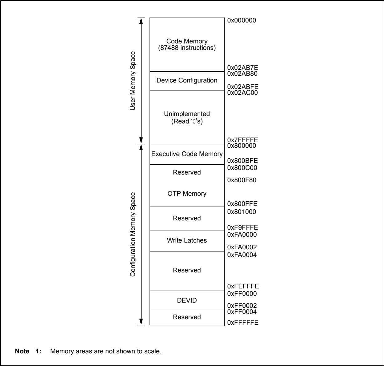
FIGURE 2-9: PROGRAM MEMORY MAP FOR dsPIC33EV256GM00X/10X DEVICES (1)
