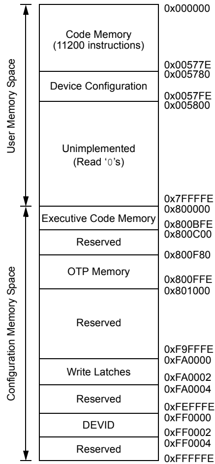
FIGURE 2-6: PROGRAM MEMORY MAP FOR dsPIC33EV32GM00X/10X DEVICES (1)
