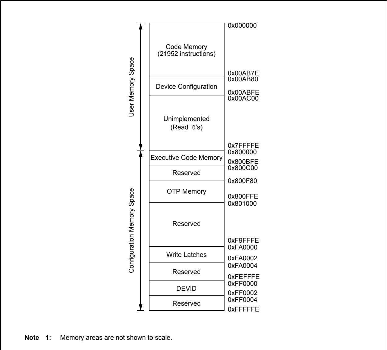
FIGURE 2-7: PROGRAM MEMORY MAP FOR dsPIC33EV64GM00X/10X DEVICES (1)
