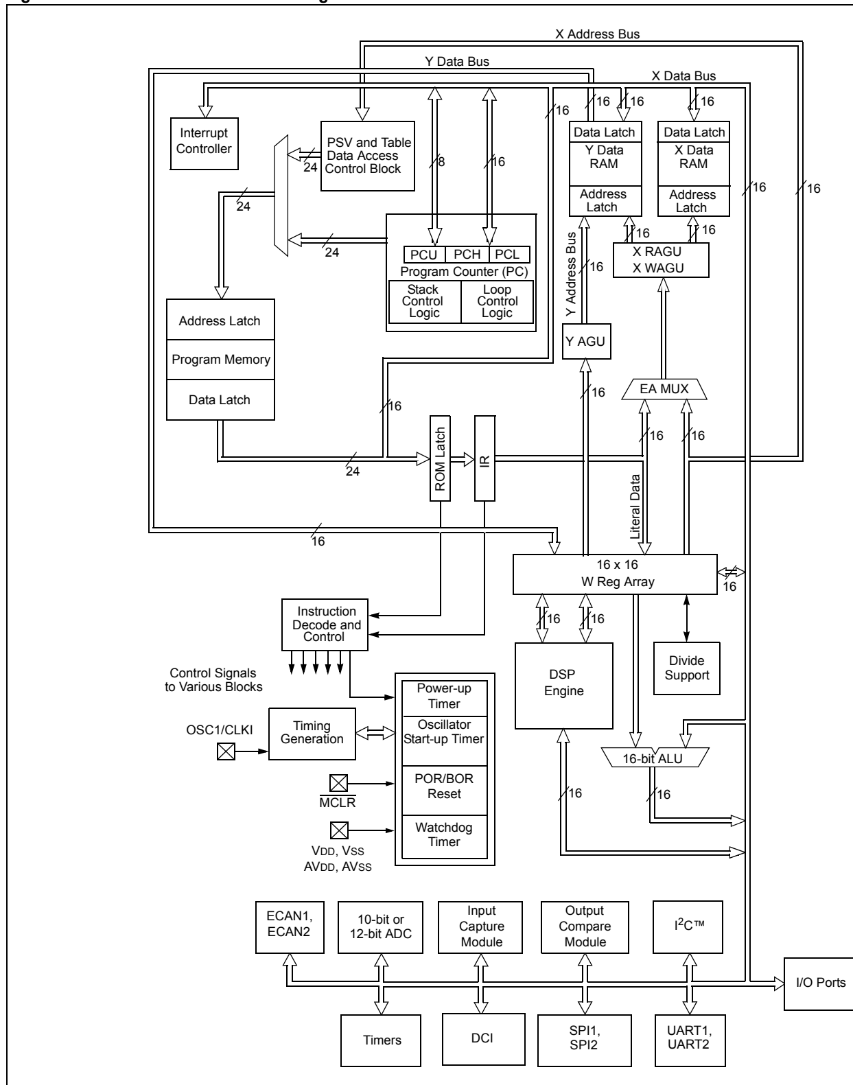
Figure 2-1: dsPIC33F CPU Block Diagram
