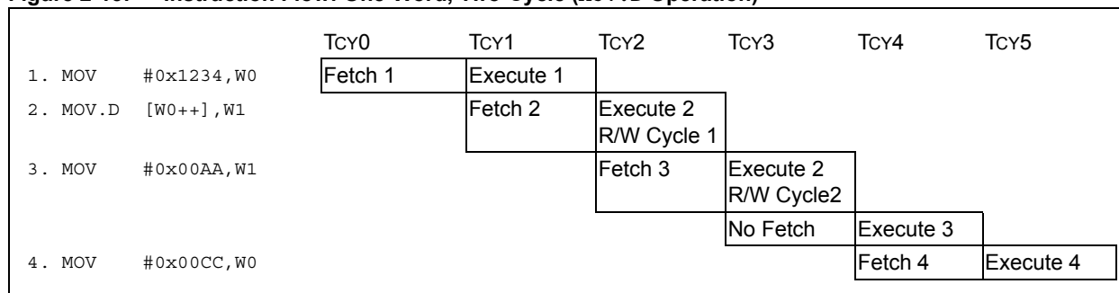
Figure 2-13: Instruction Flow: One-Word, Two-Cycle (MOV.D Operation)
