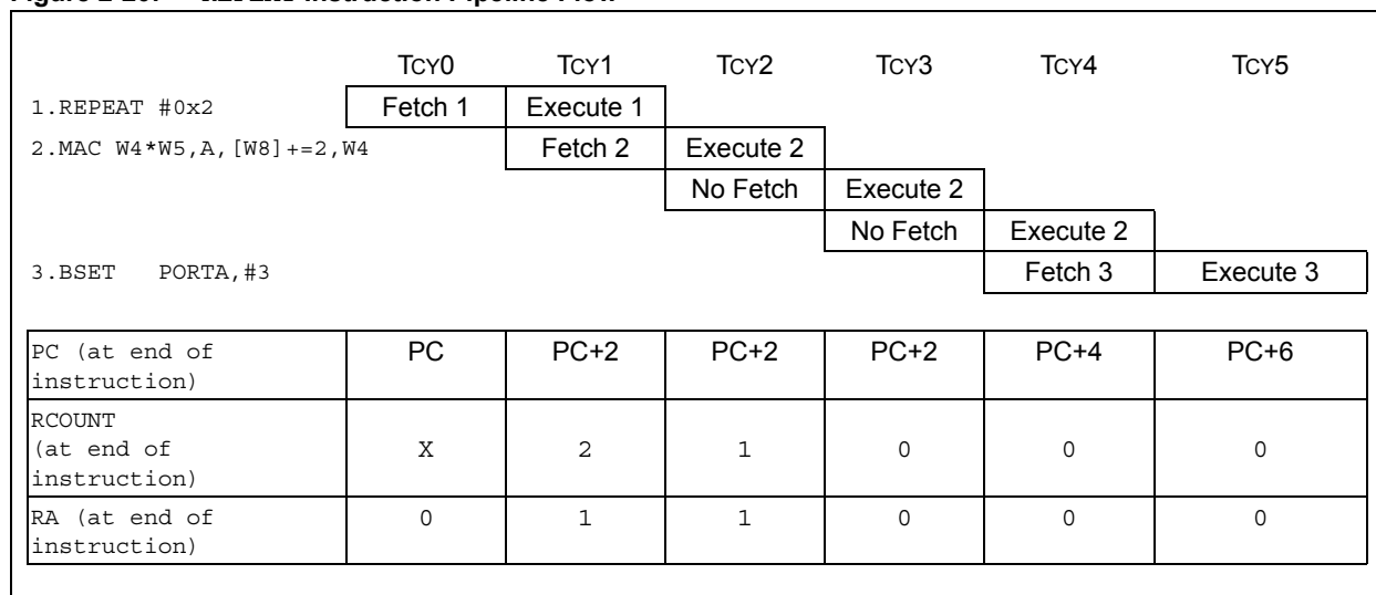
Figure 2-20: REPEAT Instruction Pipeline Flow
