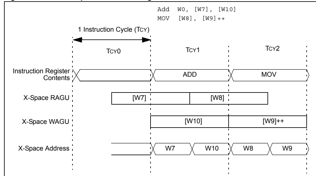
Figure 2-21: Data Space Access Timing
