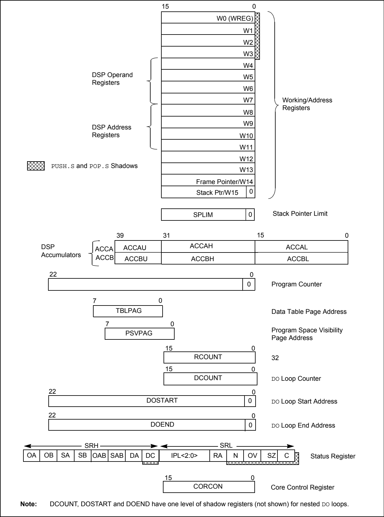
Figure 2-2: Programmer's Model
