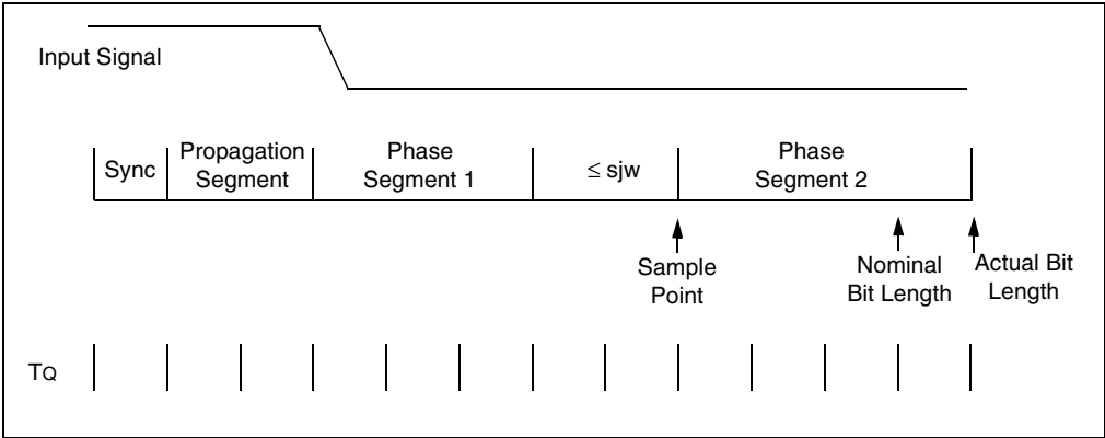
Figure 23-21: Lengthening a Bit Period
