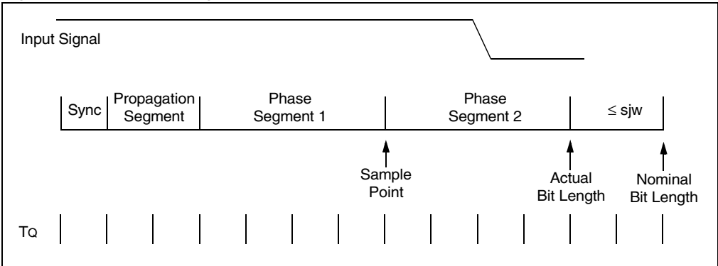
Figure 23-22: Shortening a Bit Period
