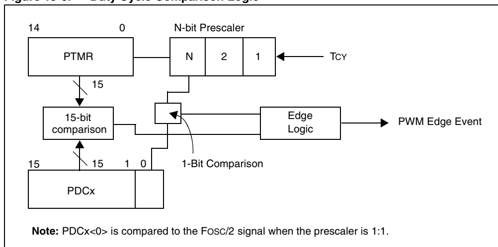
Figure 15-6: Duty Cycle Comparison Logic
