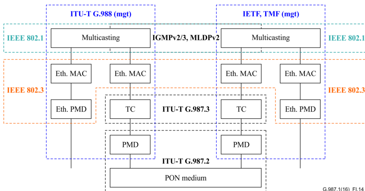
Figure I.14 – Multicast service
