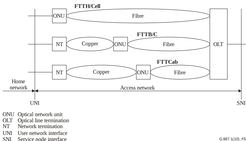
Figure 5-1 – Network architecture
