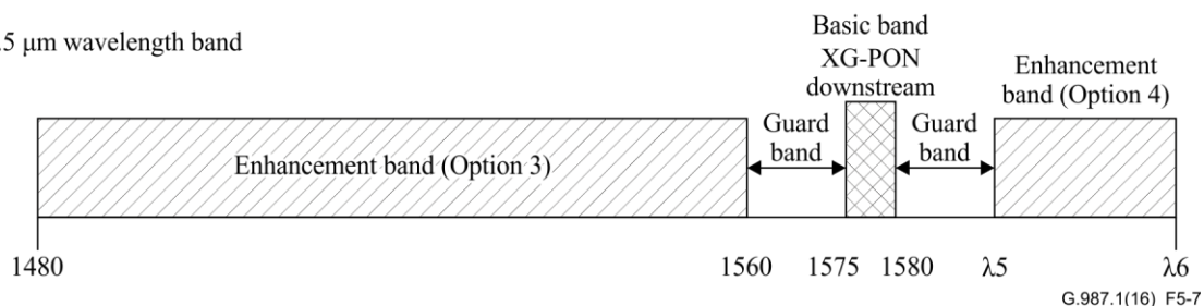
Figure 5-7 – Wavelength allocation
