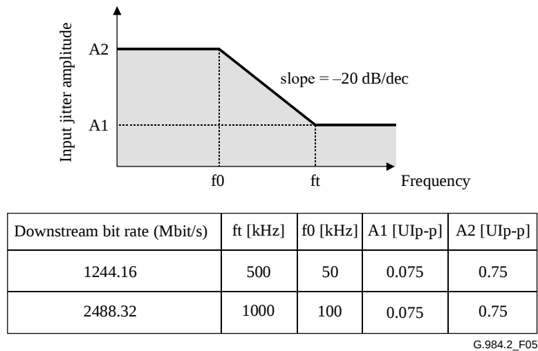
Figure 5 – Jitter tolerance mask for ONU
