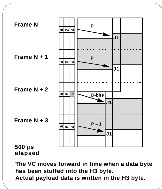
► Figure 11. Payload pointer – negative justification.
