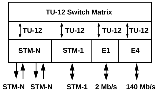
► Figure 22. Wideband digital cross-connect example.
