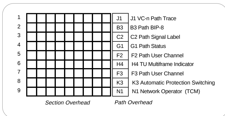
► Figure 7. Higher-order path overhead (VC-4/VC-3).
