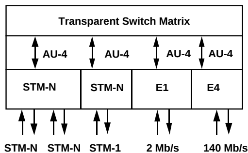
► Figure 23. Broadband digital cross-connect example.
